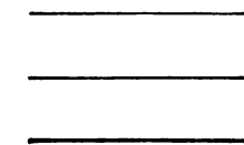
FIG. 24. — The actual thickness of the chlorenchyma of leaves, as seen in cross section.
